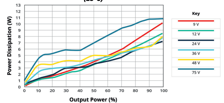
POWER DISSIPATION VS OUTPUT POWER PRQE75W-E12-S48-D (25°C)
