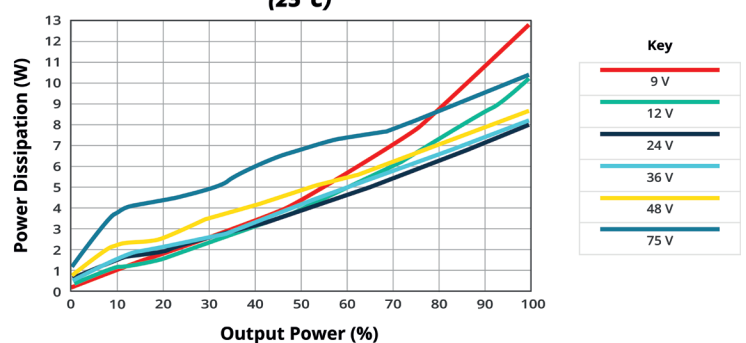
POWER DISSIPATION VS OUTPUT POWER PRQE75W-E12-S15-D (25°C)
