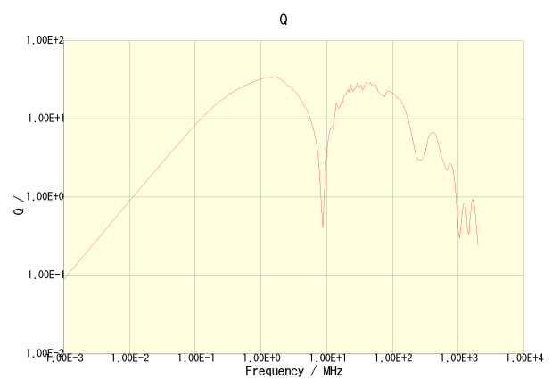
NLV32T-221J-EF
