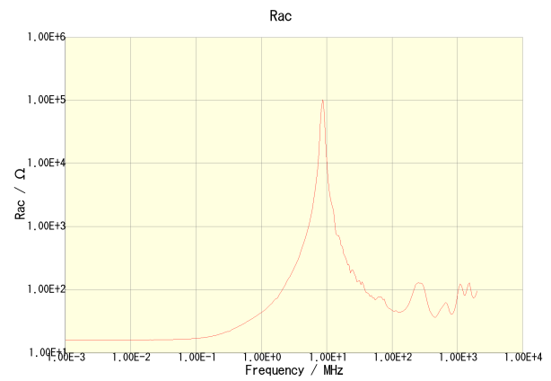
NLV32T-221J-EF
