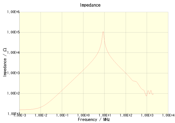
NLV32T-221J-EF
