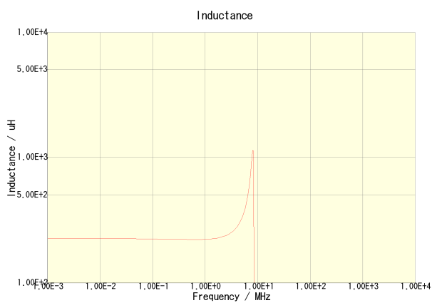
NLV32T-221J-EF
