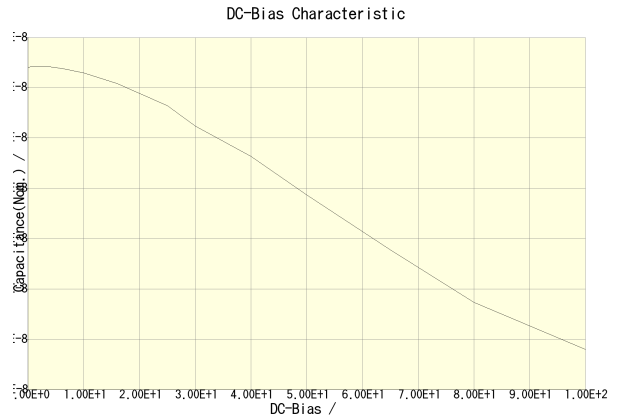
C2012X7R2A473K125AA
