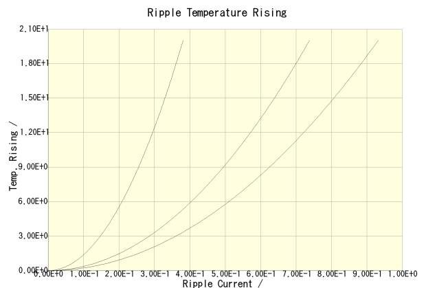
C2012X7R2A473K125AA(100kHz) C2012X7R2A473K125AA(500kHz) C2012X7R2A473K125AA(1MHz)
