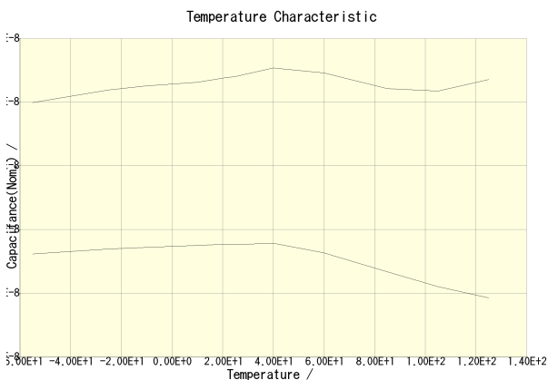
C2012X7R2A473K125AA(DC Bias = 0V) C2012X7R2A473K125AA(DC Bias = 50V)
