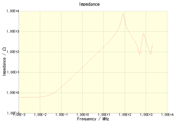
NLV32T-2R7J-PF
