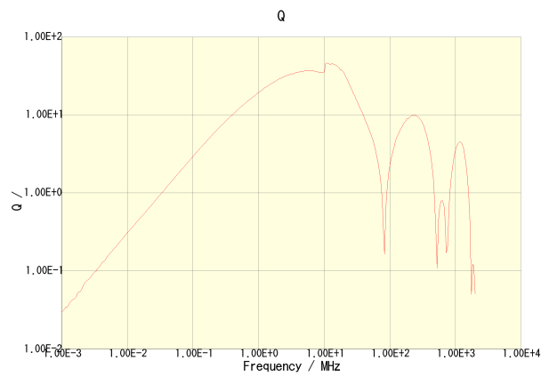
NLV32T-2R7J-PF
