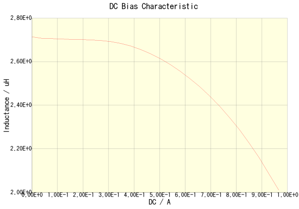
NLV32T-2R7J-PF(Amb. Temp. = 20degc)
