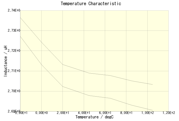
NLV32T-2R7J-PF(DC = 0A)
