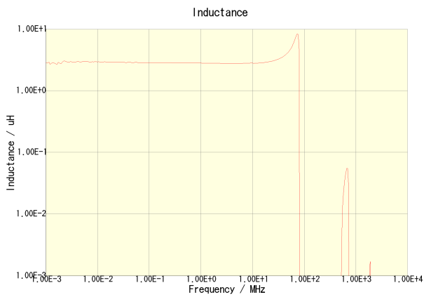
NLV32T-2R7J-PF
