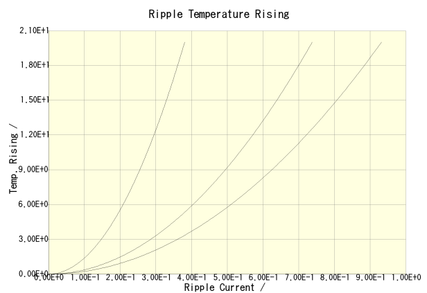
C2012X7R2A473K125AA(100kHz) C2012X7R2A473K125AA(500kHz) C2012X7R2A473K125AA(1MHz)
