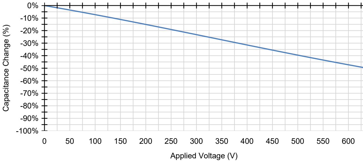
VCC Characterization
