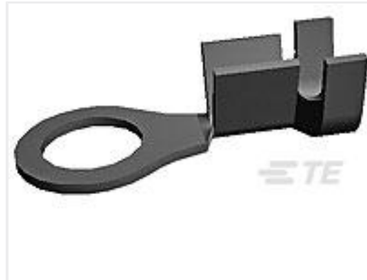
TE Part #40696 RING TERMINAL 12-10 AWG TPBR
