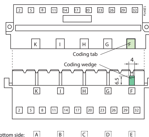
Fig. 18 Integrated code key system (H11 connector)
