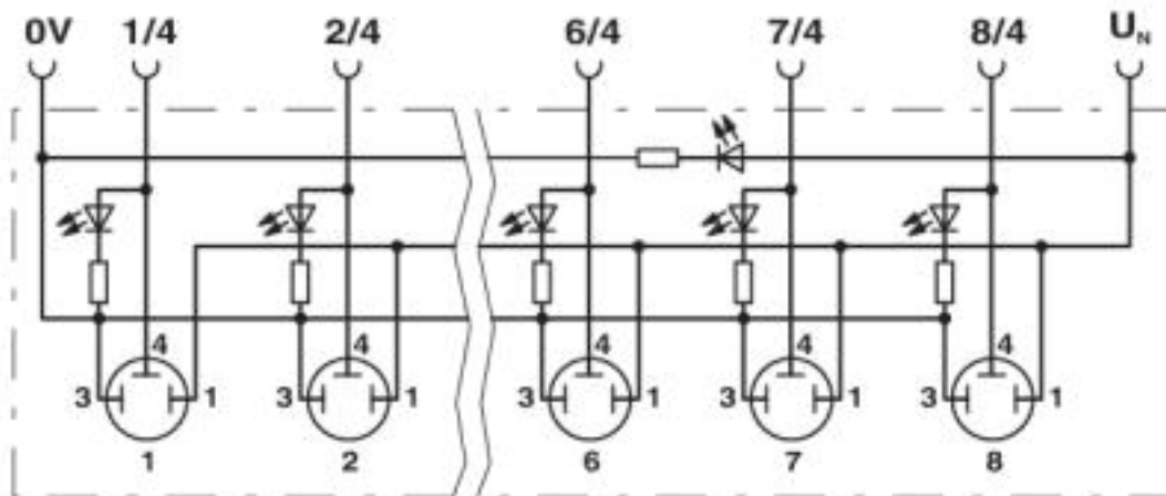
Circuit diagram
