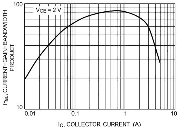
Figure 7. Current-Gain-Bandwidth Product
