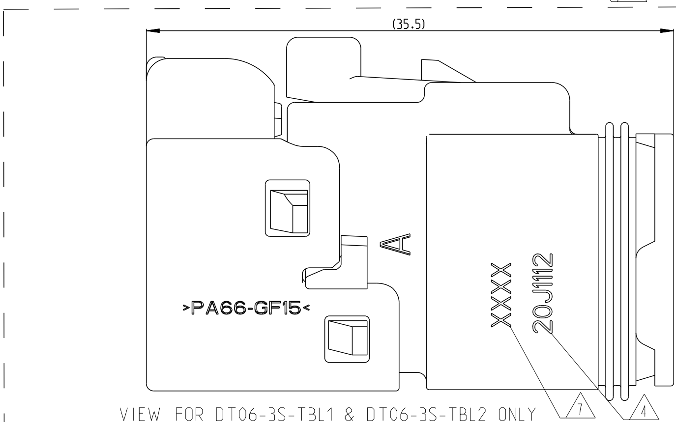
VIEW FOR DT06-3S-TBL1 & DT06-3S-TBL2 ONLY
