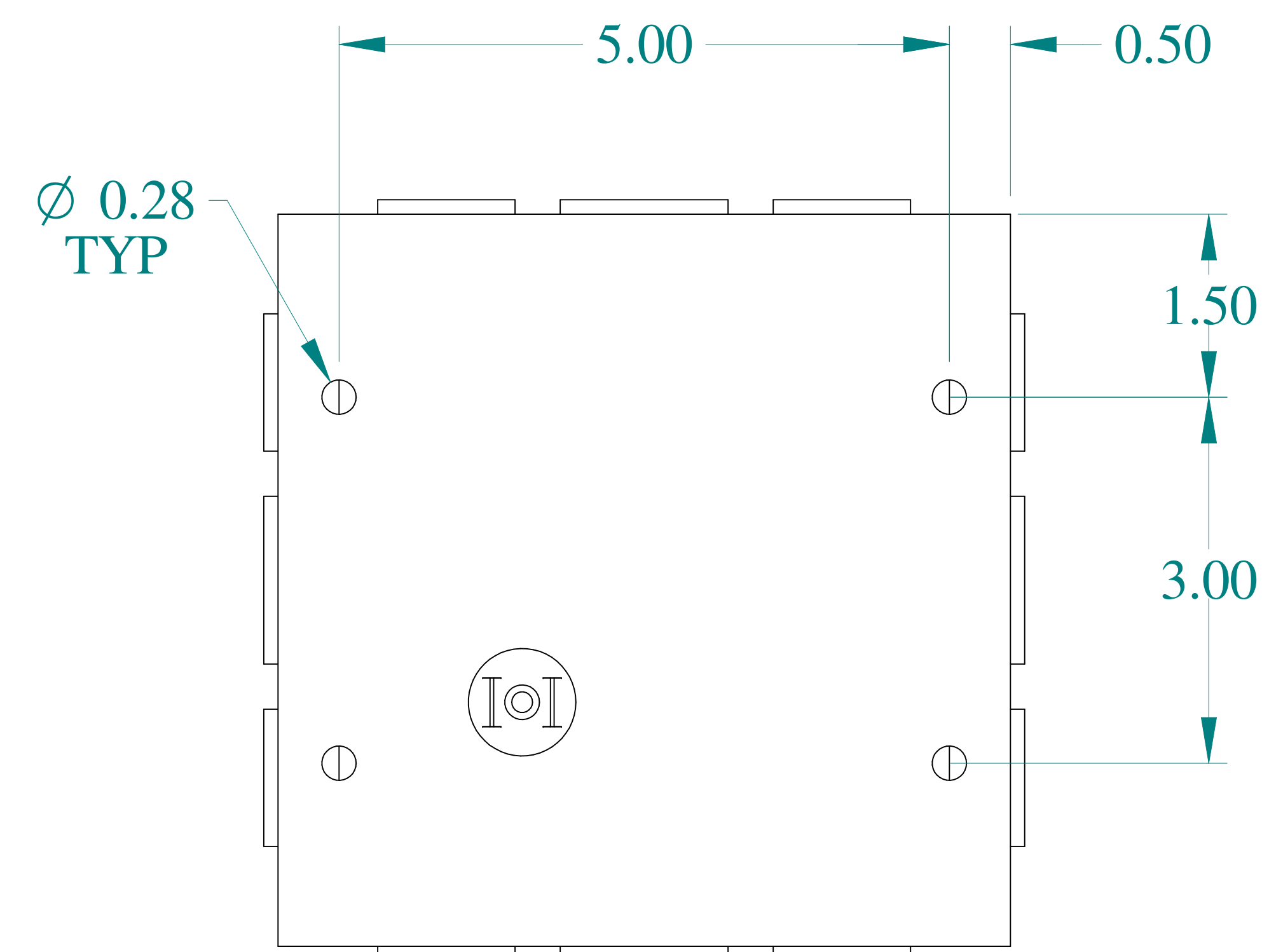
BOTTOM VIEW
