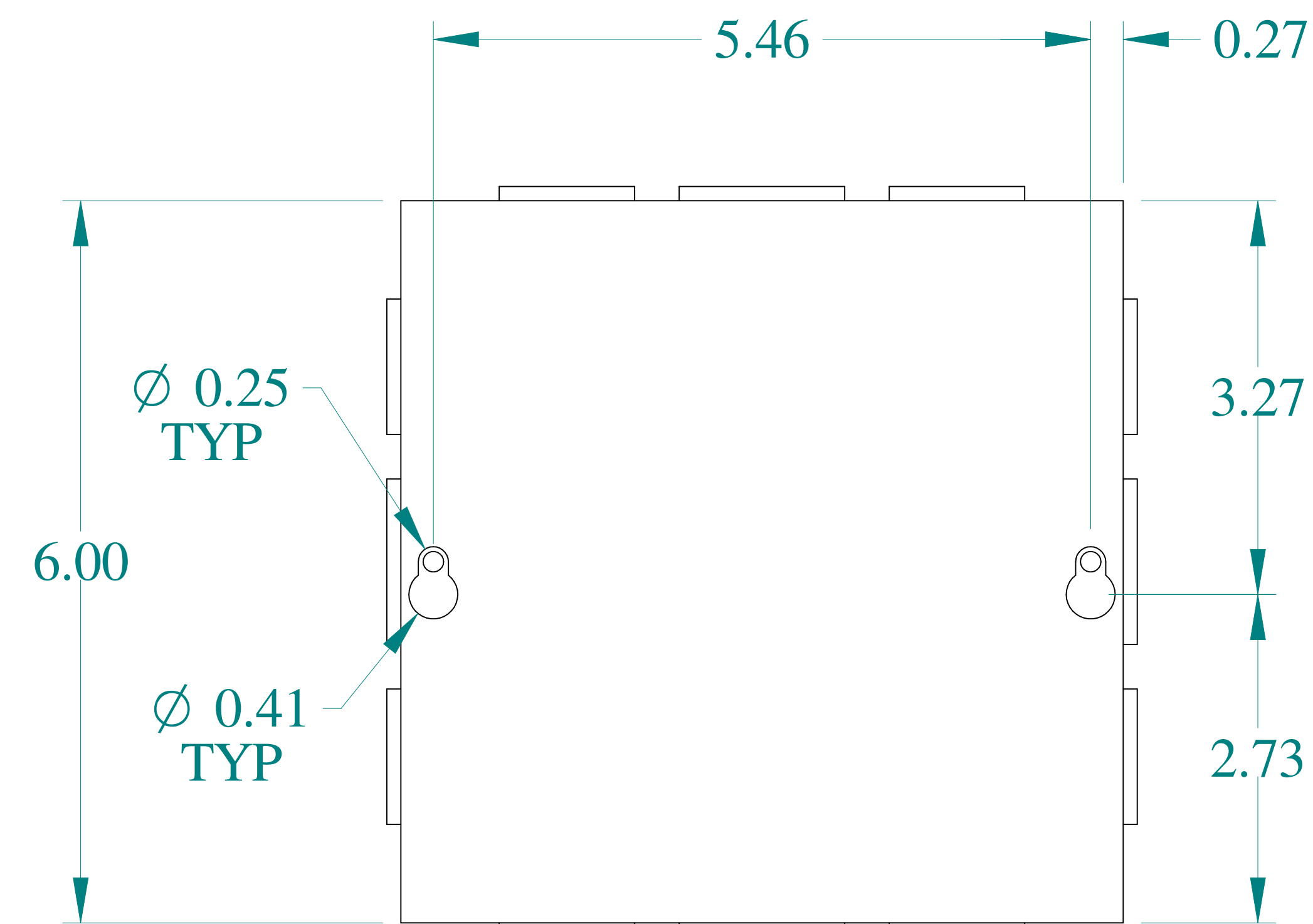
TOP VIEW
