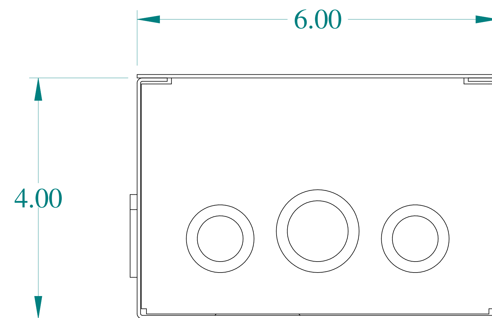
FRONT VIEW
