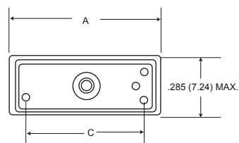
Face View
