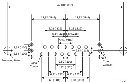
Shell Size Contact Arrangement No. of Size 20 Cavities No. of Size 8 Cavities B 17W2 15 #20 2 #8
