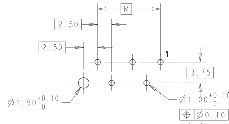
PCB LAYOUT A - SOLDER SIDE ODD NUMBER OF PINS
