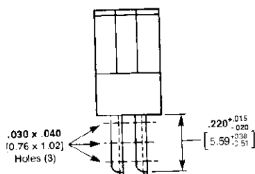
Solder Eyelet Contact Max. Wire Size, 26 AWG (0.15 mm 2 )
