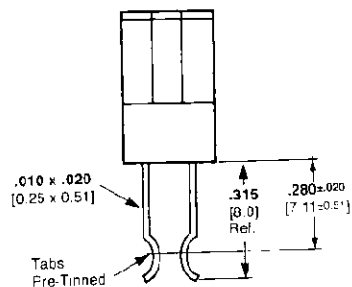
Card Extender Contact (Use with .070/.054 [1.78/1.37] Board)
