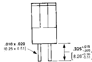
.010 x .020 [0.25 x 0.51] Posted Contact 1
