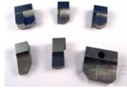
TE Part #4-1333206-3 ANVIL, COMBINATION (.100)
