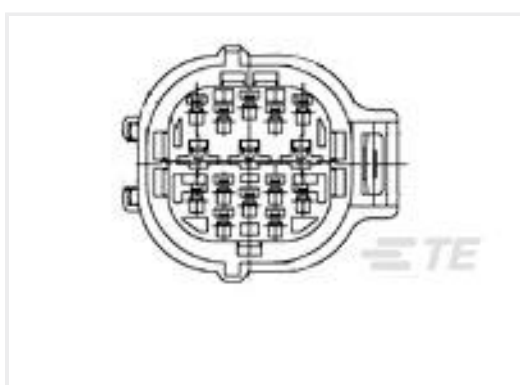
TE Part #2-85262-1 E-S MK-2(+) 15P PLUG ASSY
